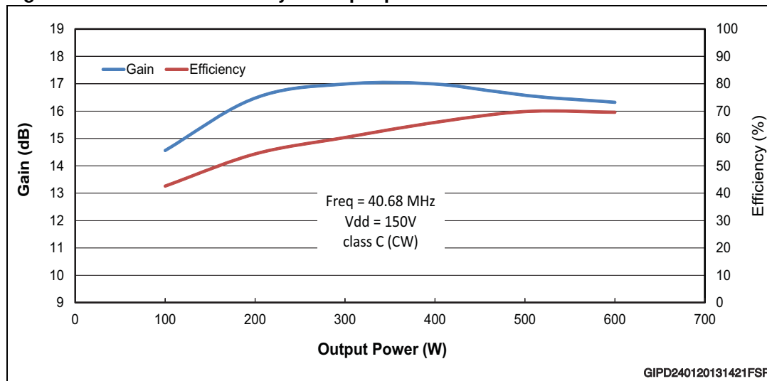
Figure 6. Gain and efficiency vs output power
