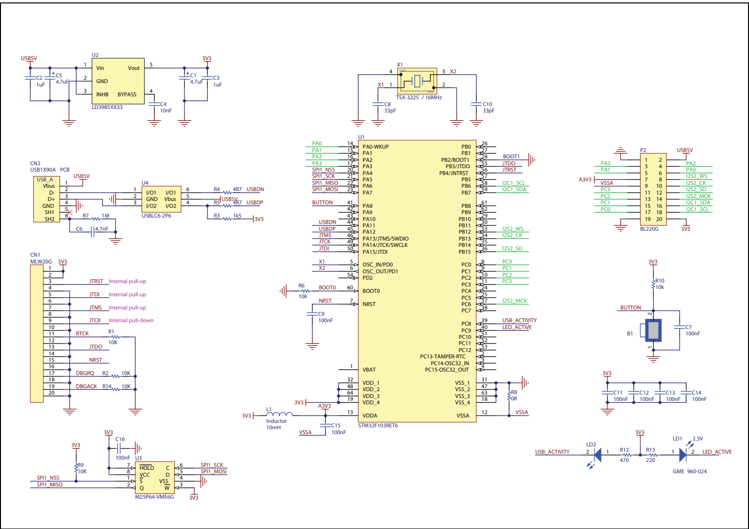
Figure 1. Schematic diagram of the STM32F103RE-based controller board
