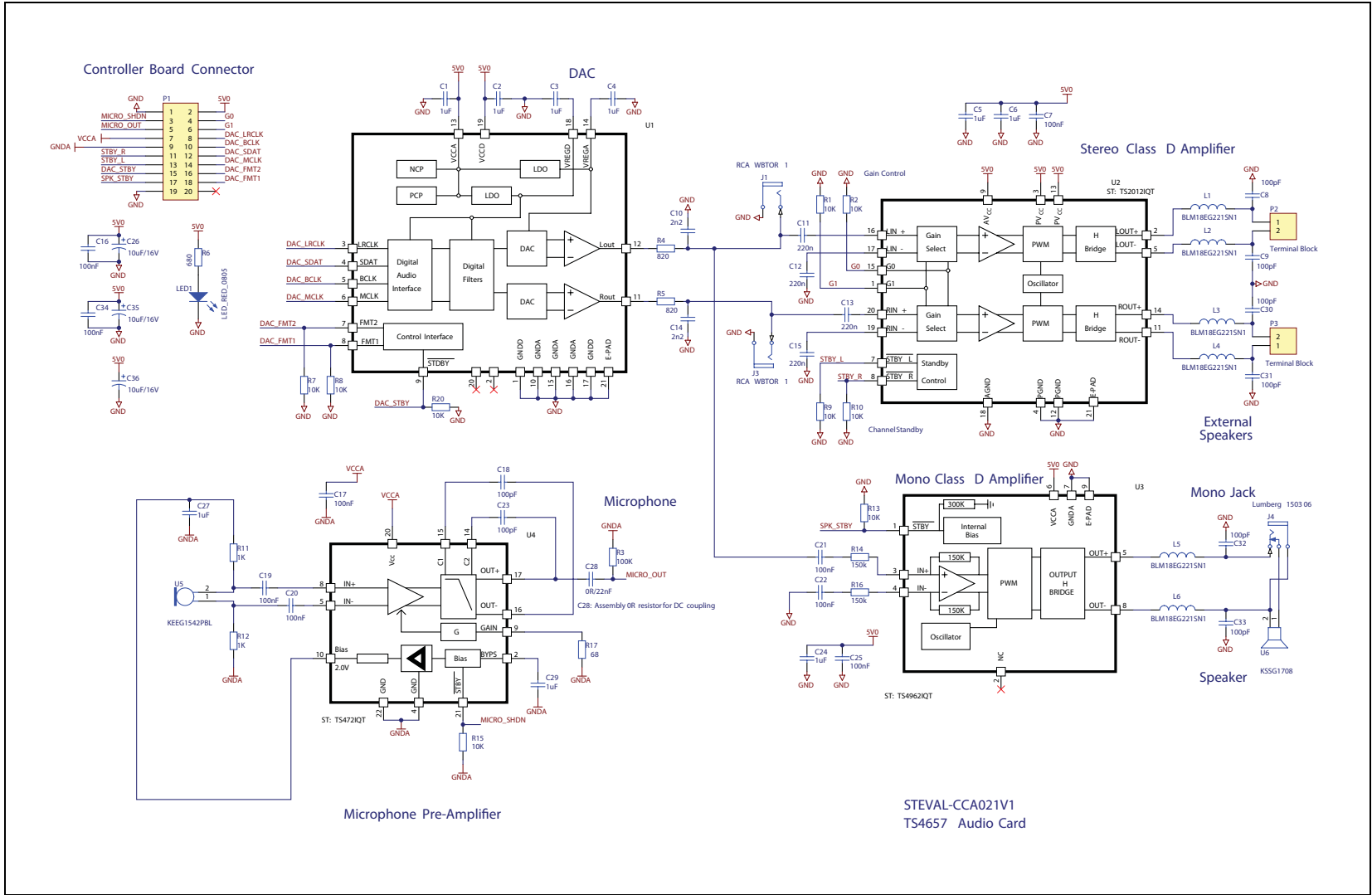
Figure 2. Schematic circuit of the TS4657-based audio board
