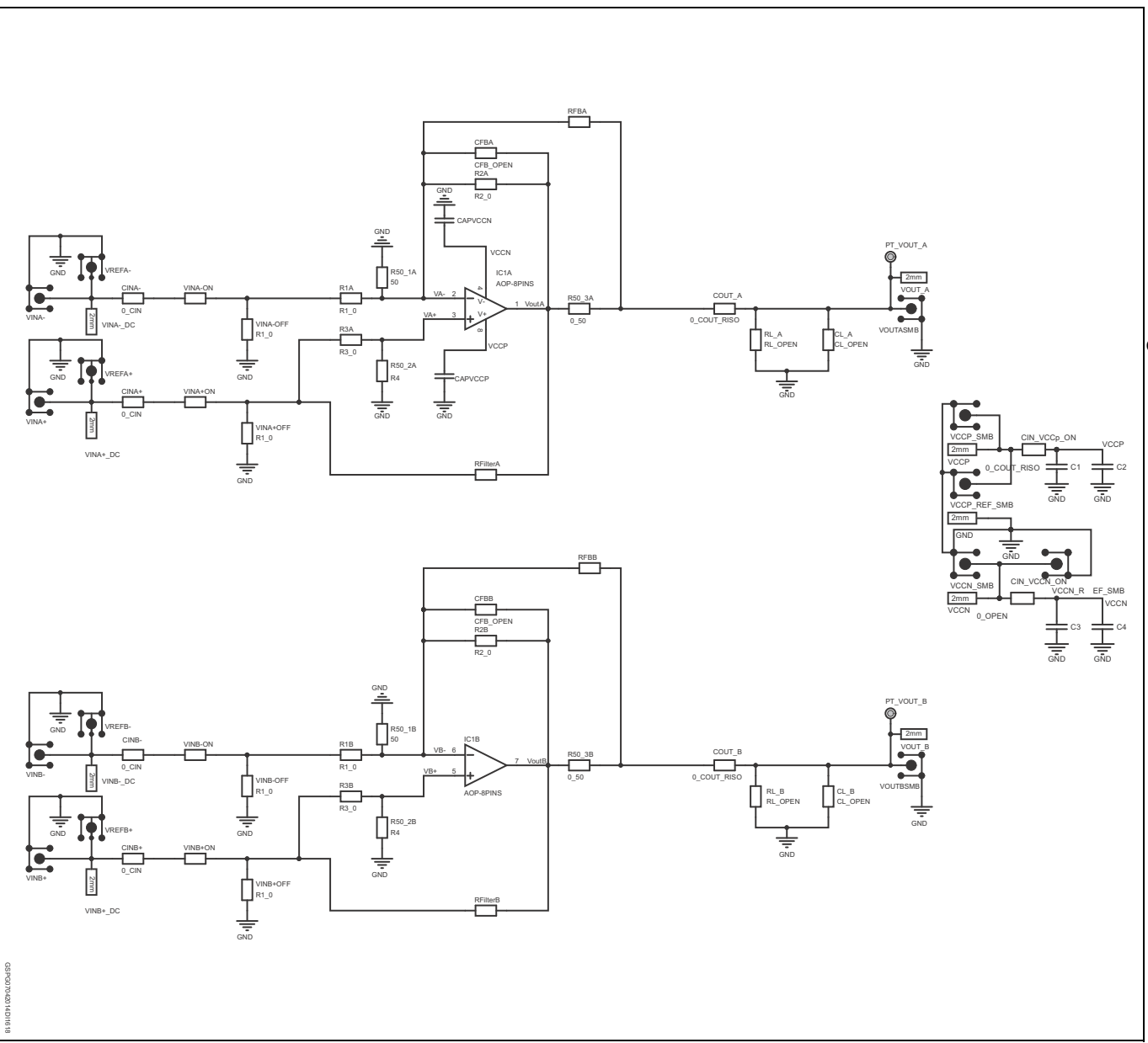
Figure 3. Evaluation board schematics
