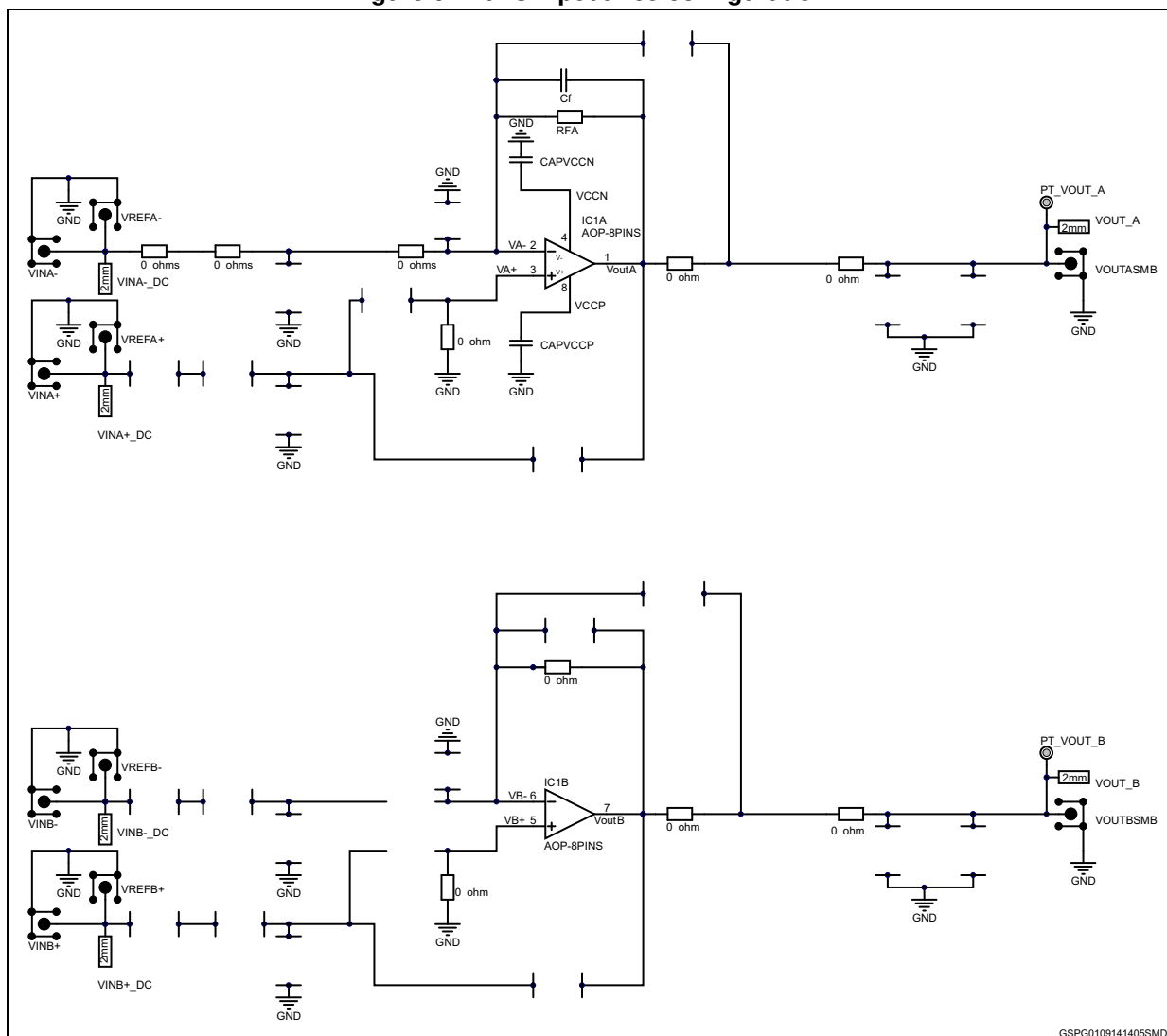
Figure 9. Transimpedance configuration
