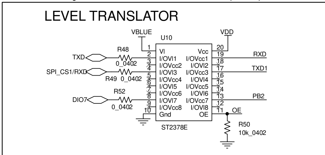
Figure 12: STEVAL-IDB008V1 circuit schematic (12 of 12)
