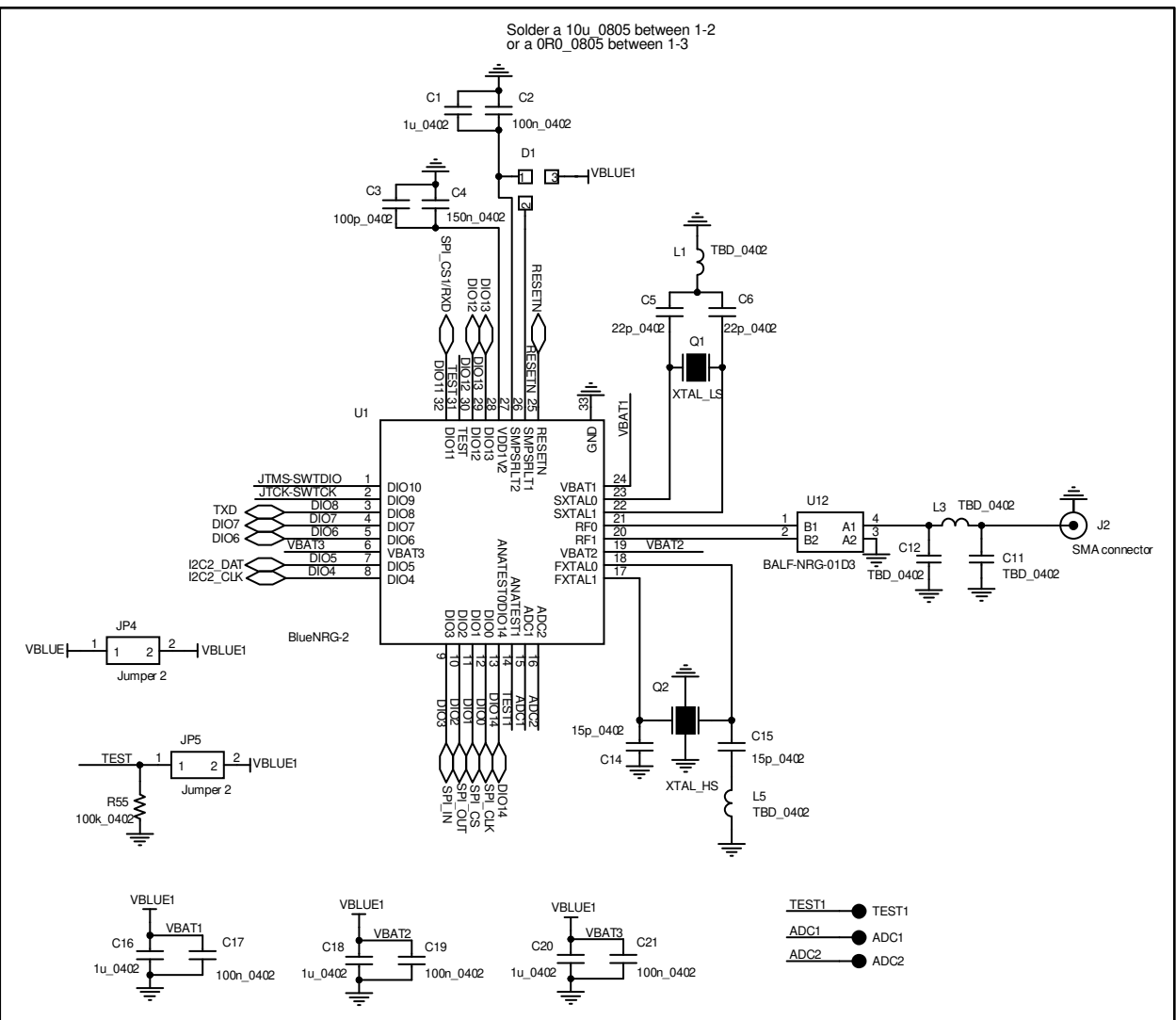
Figure 3: STEVAL-IDB008V1 circuit schematic (3 of 12)
