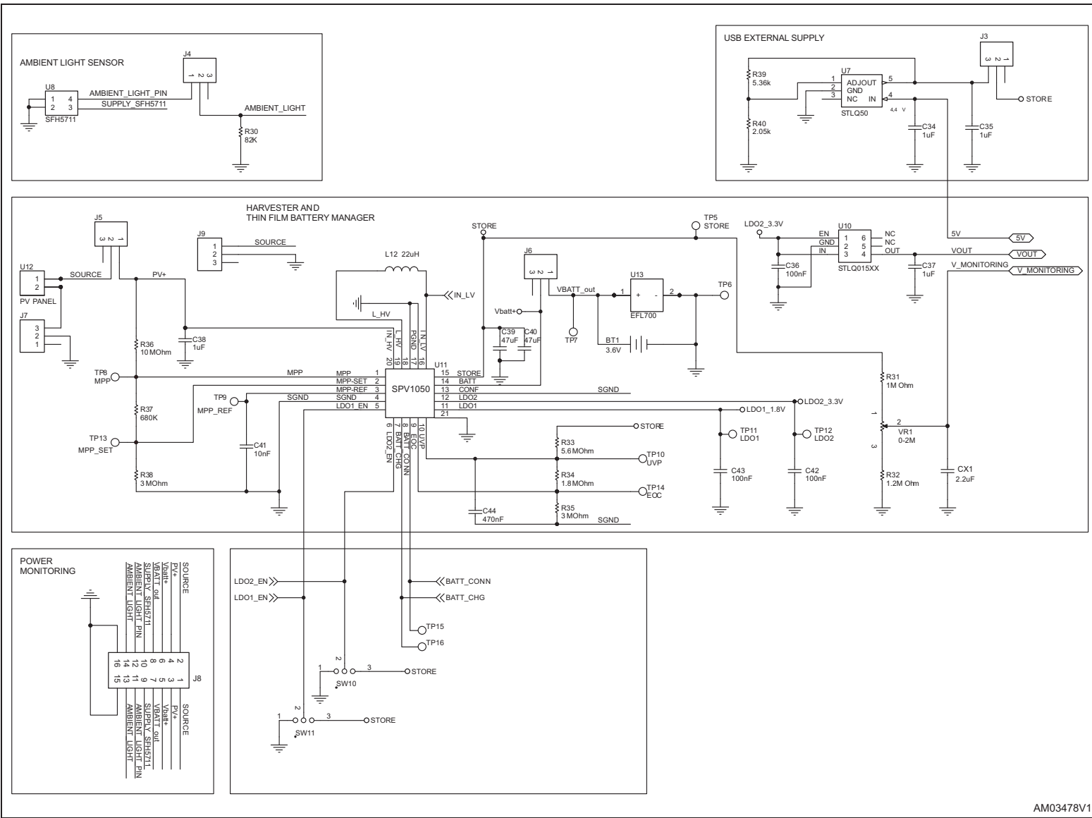
Figure 4. Board schematic - photovoltaic harvester
