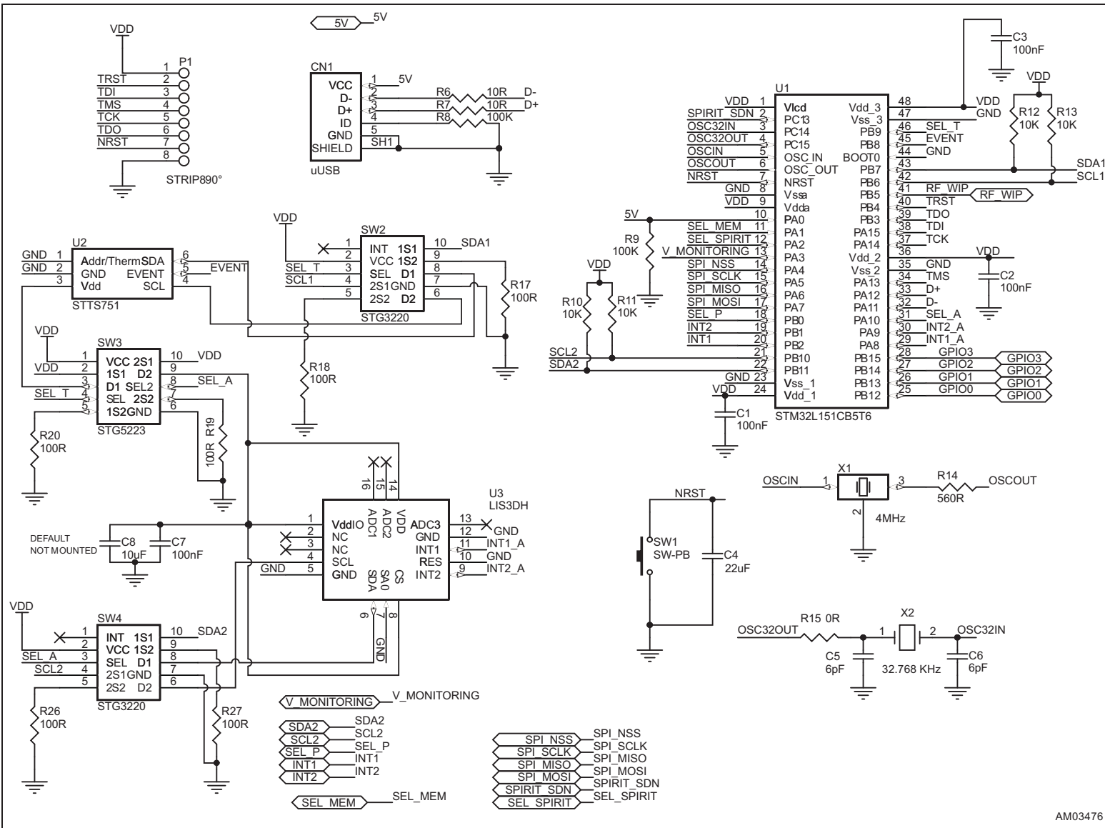
Figure 3. Board schematic - microcontroller
