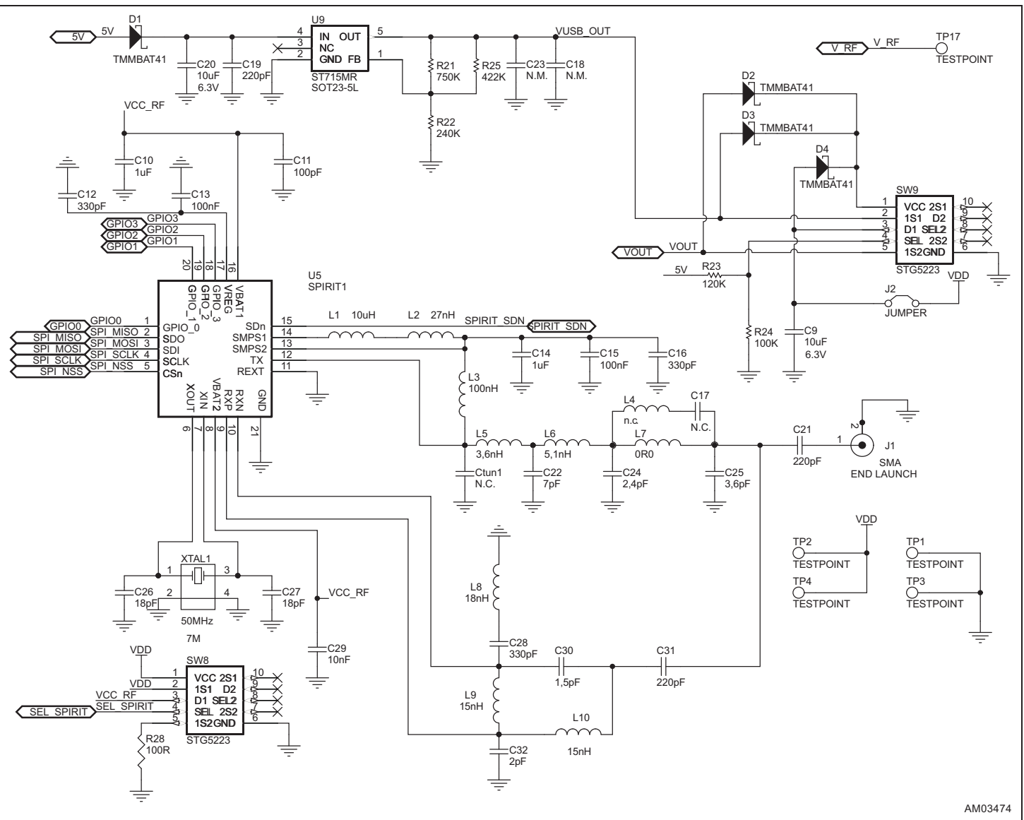
Figure 1. Board schematic - transmitter/receiver
