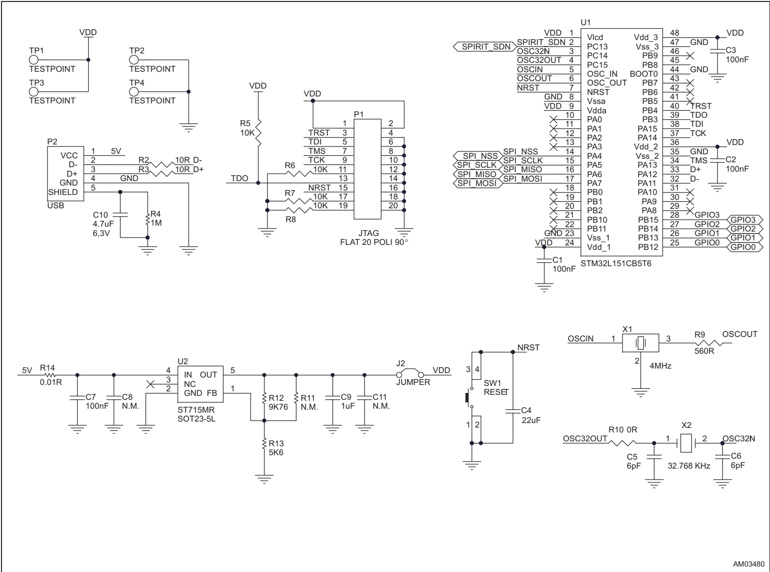
Figure 10. Receiver board schematic - microcontroller
