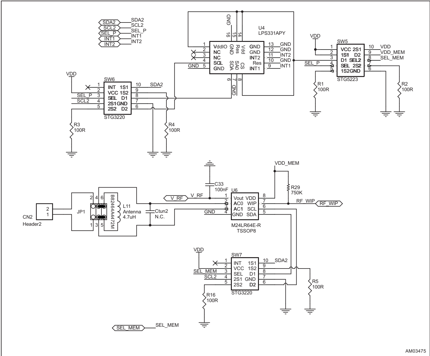
Figure 2. Board schematic - antenna
