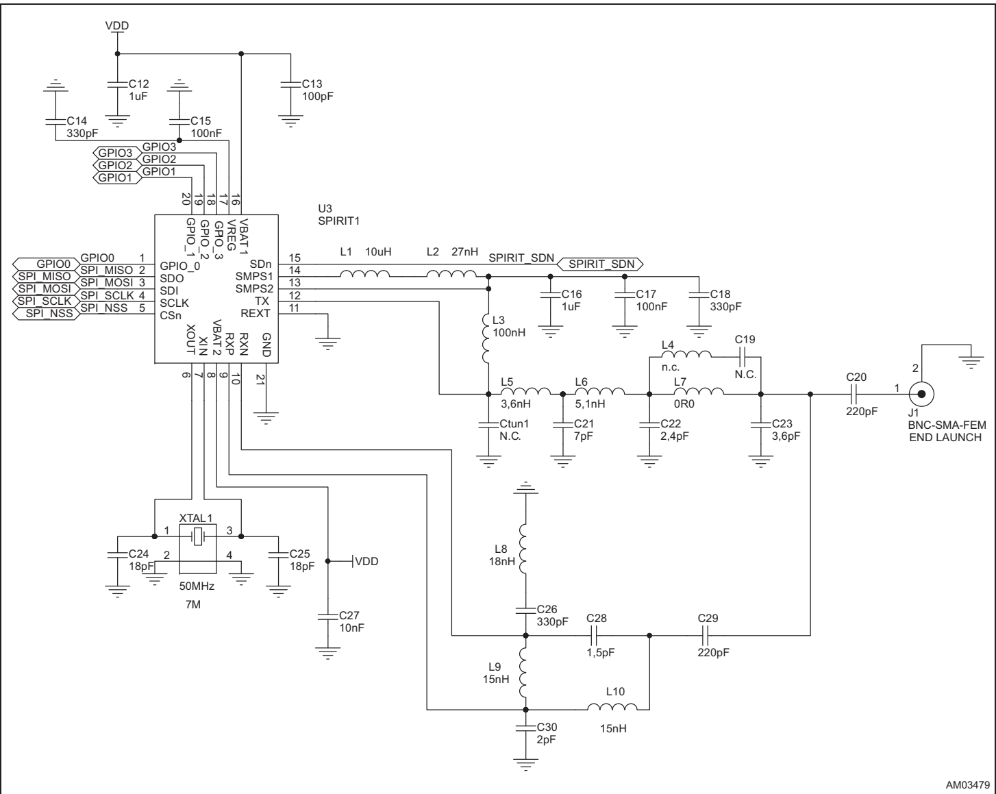
Figure 9. Receiver board schematic - RF transmitter/receiver
