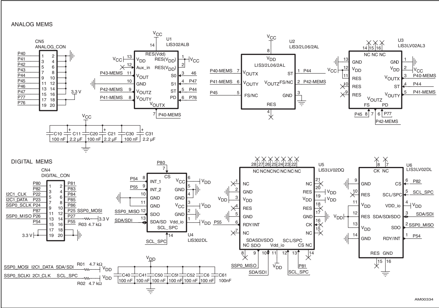
Figure 3. Schematics - analog and digital MEMS
