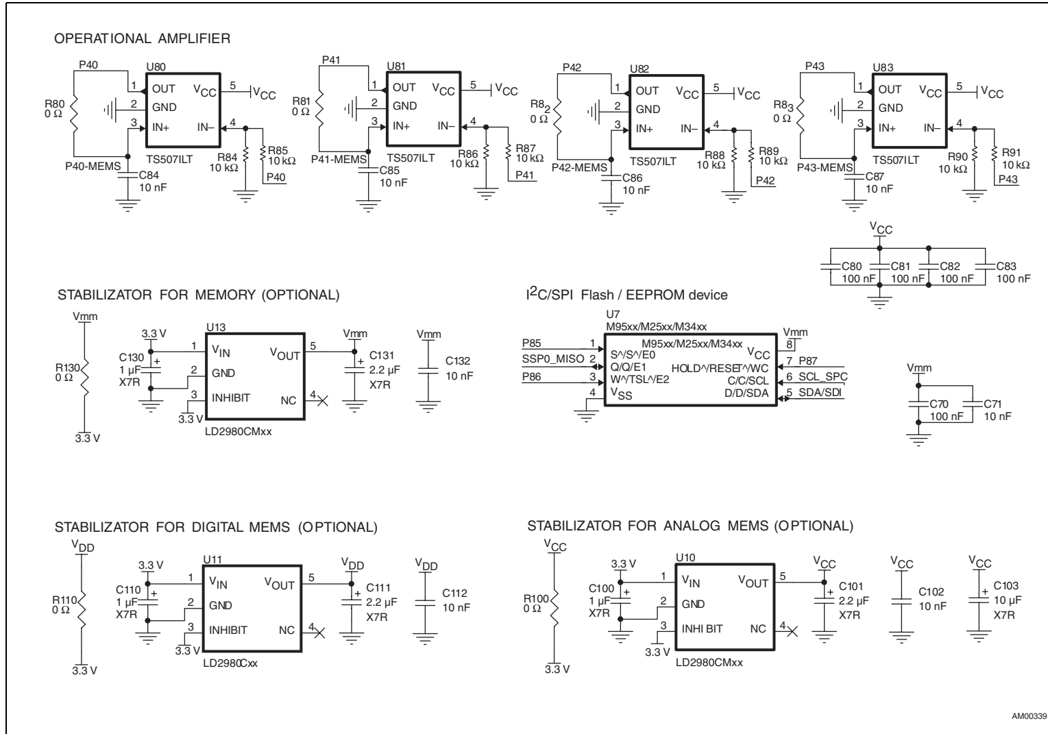
Figure 4. Schematics - I 2 C/SPI Flash/EEPROM device, amplifier, stabilizers
