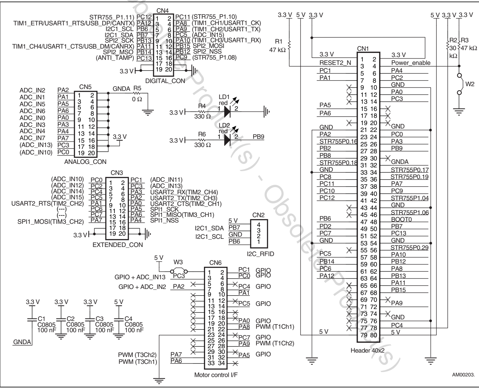
Figure 1. Interconnection board for the STM32 PerformanceStick
