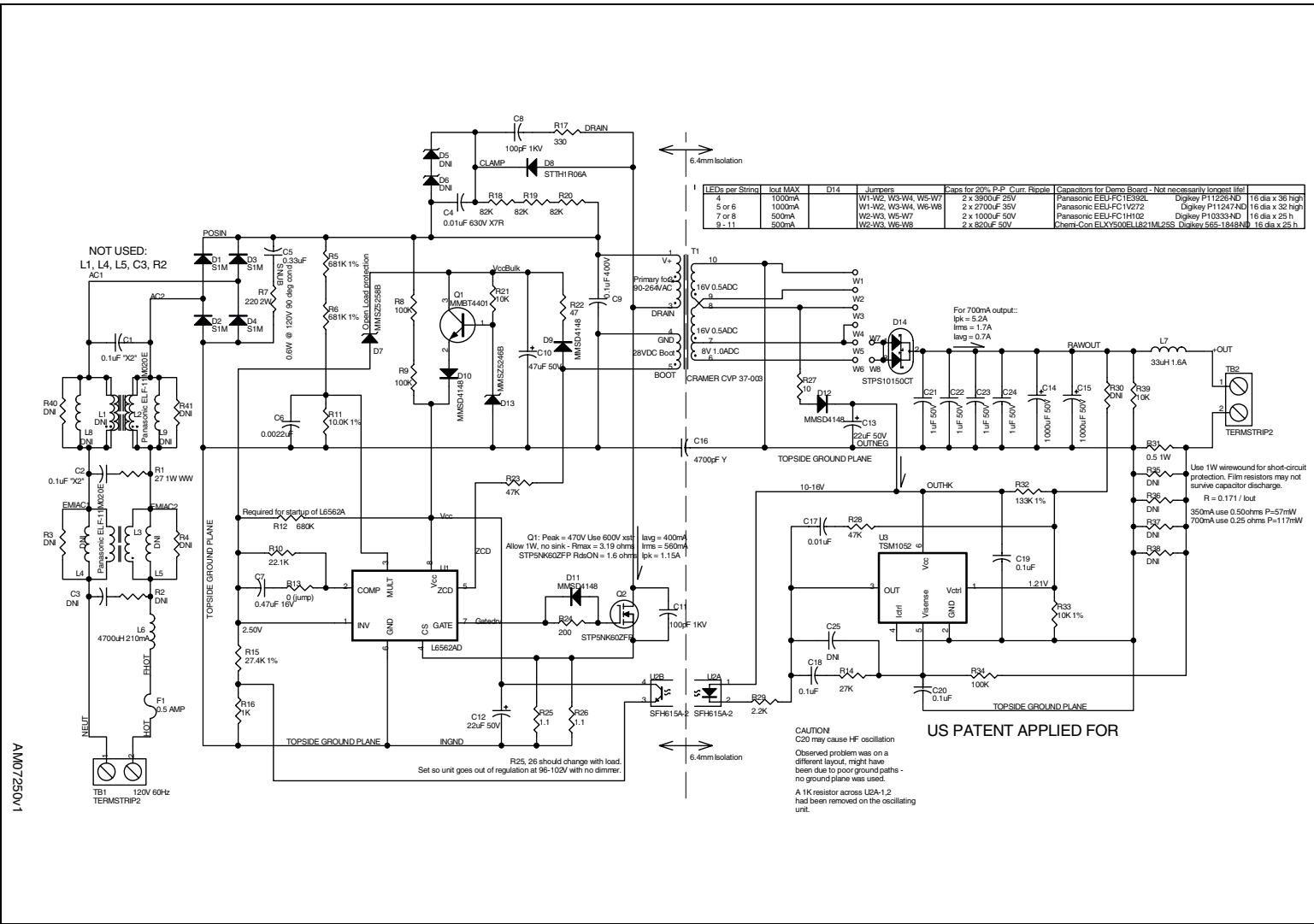
Figure 1. STEVAL-ILL016V2 circuit schematic
