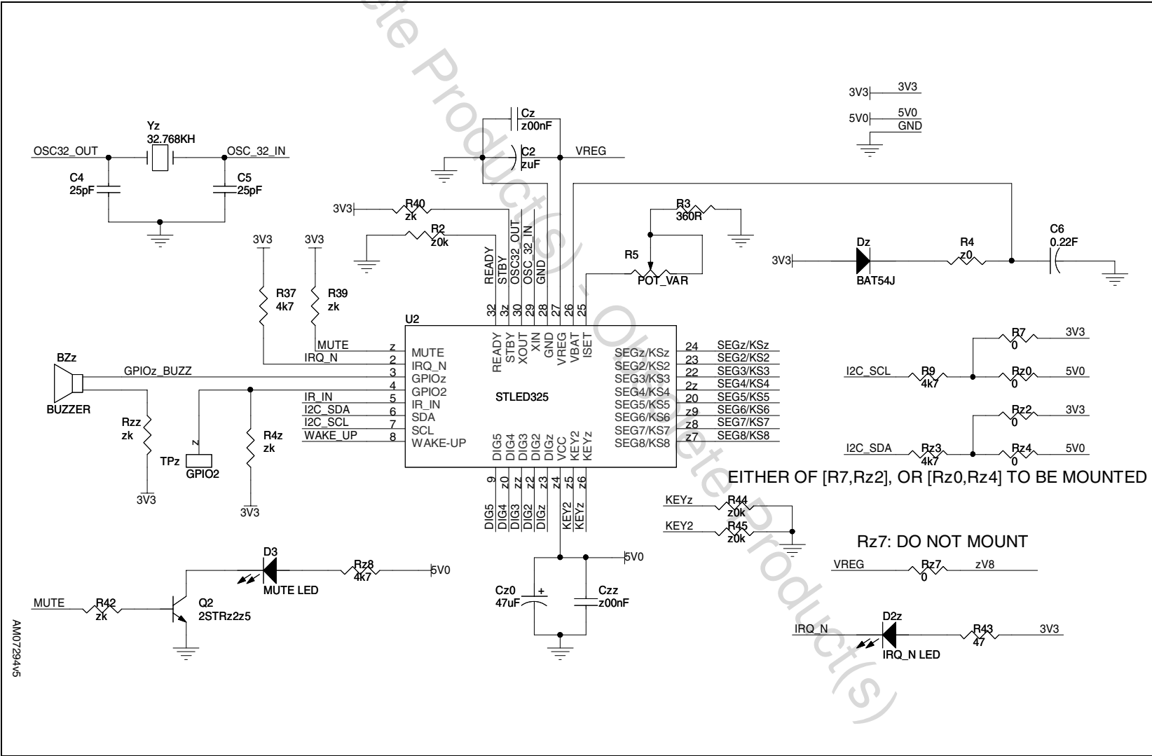
Figure 3. STEVAL-ILL029V: STLED325
