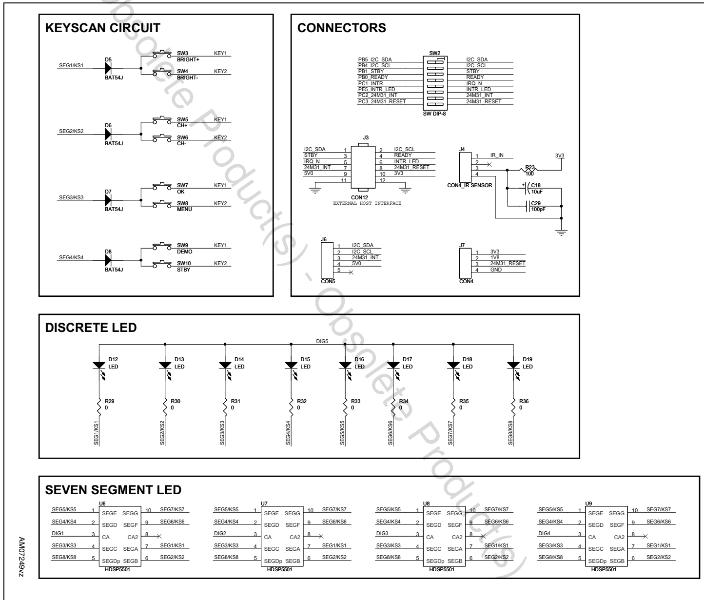
Figure 4. STEVAL-ILL029V: other blocks
