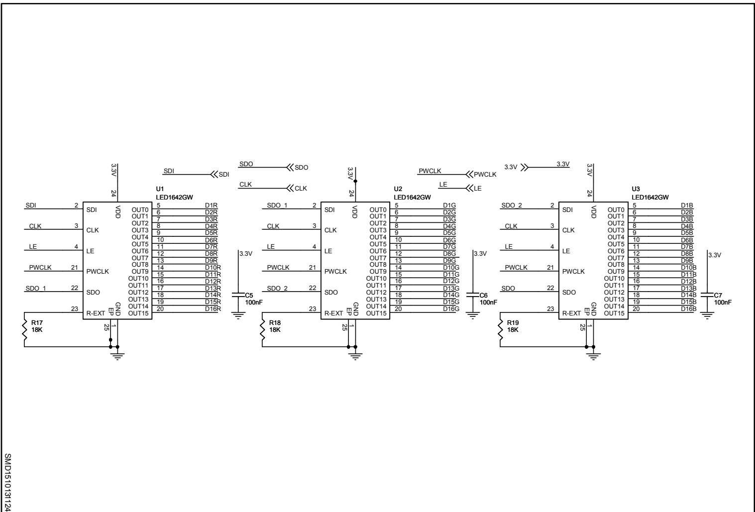
Figure 2: STEVAL-ILL061V1 LED drivers
