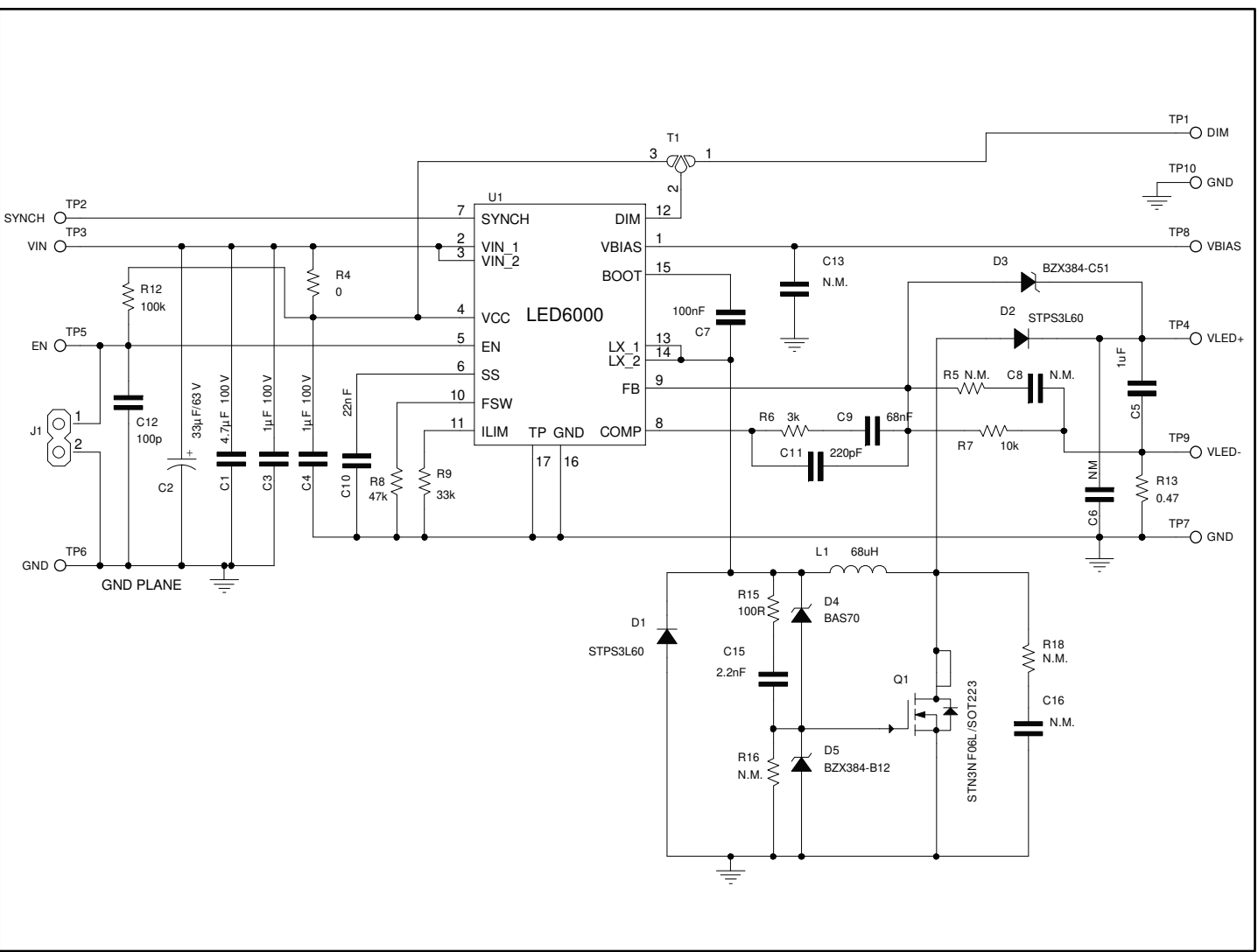
Figure 1 : STEVAL-ILL088V1 circuit schematic
