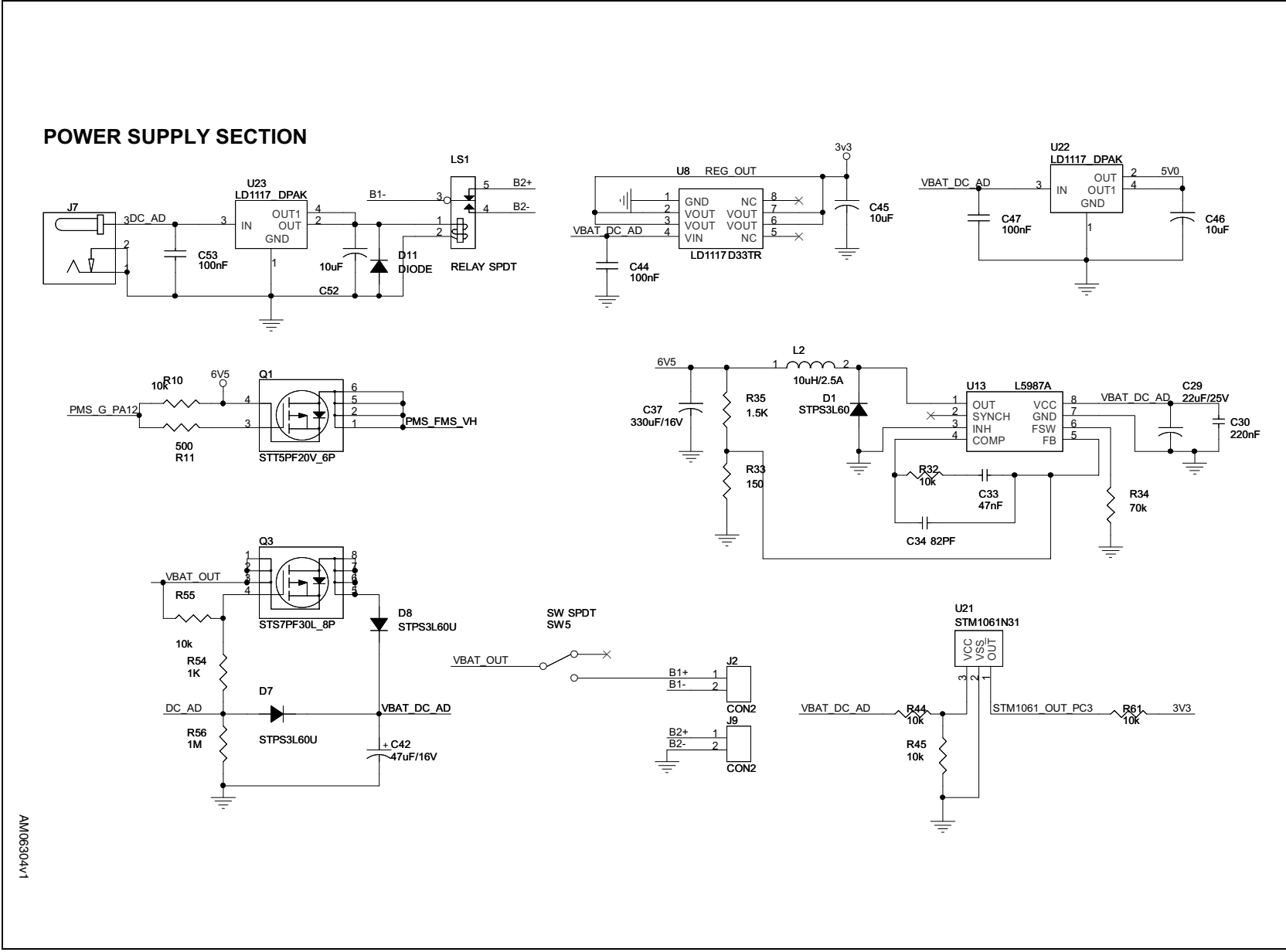
Figure 4. Power management section schematic
