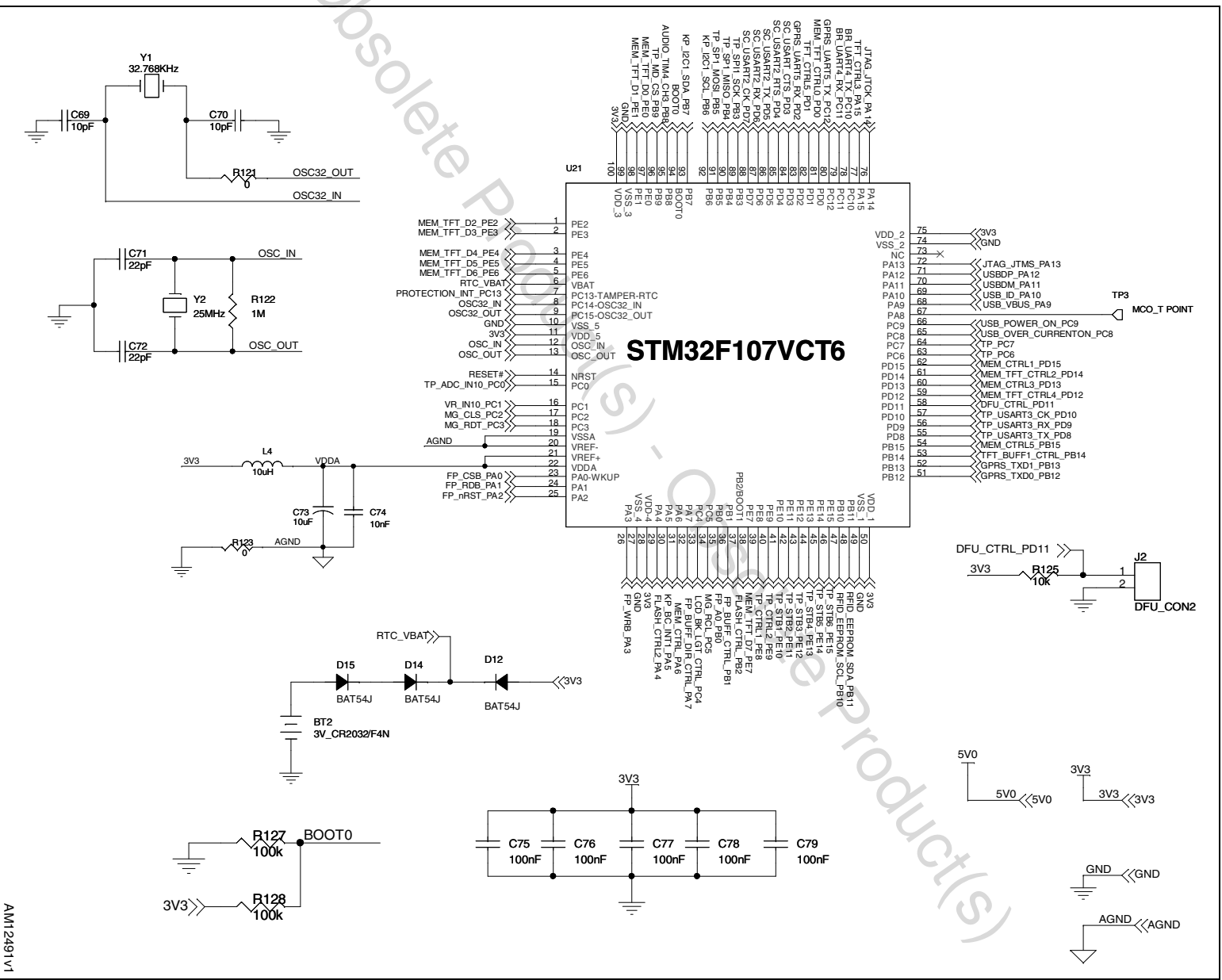
Figure 1. Schematic diagram (1 of 11)
