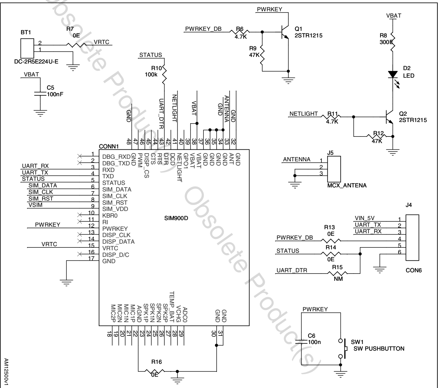
Figure 11. Schematic diagram (11 of 11)
