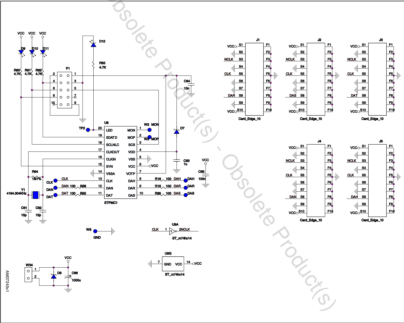
Figure 1. Circuit schematic
