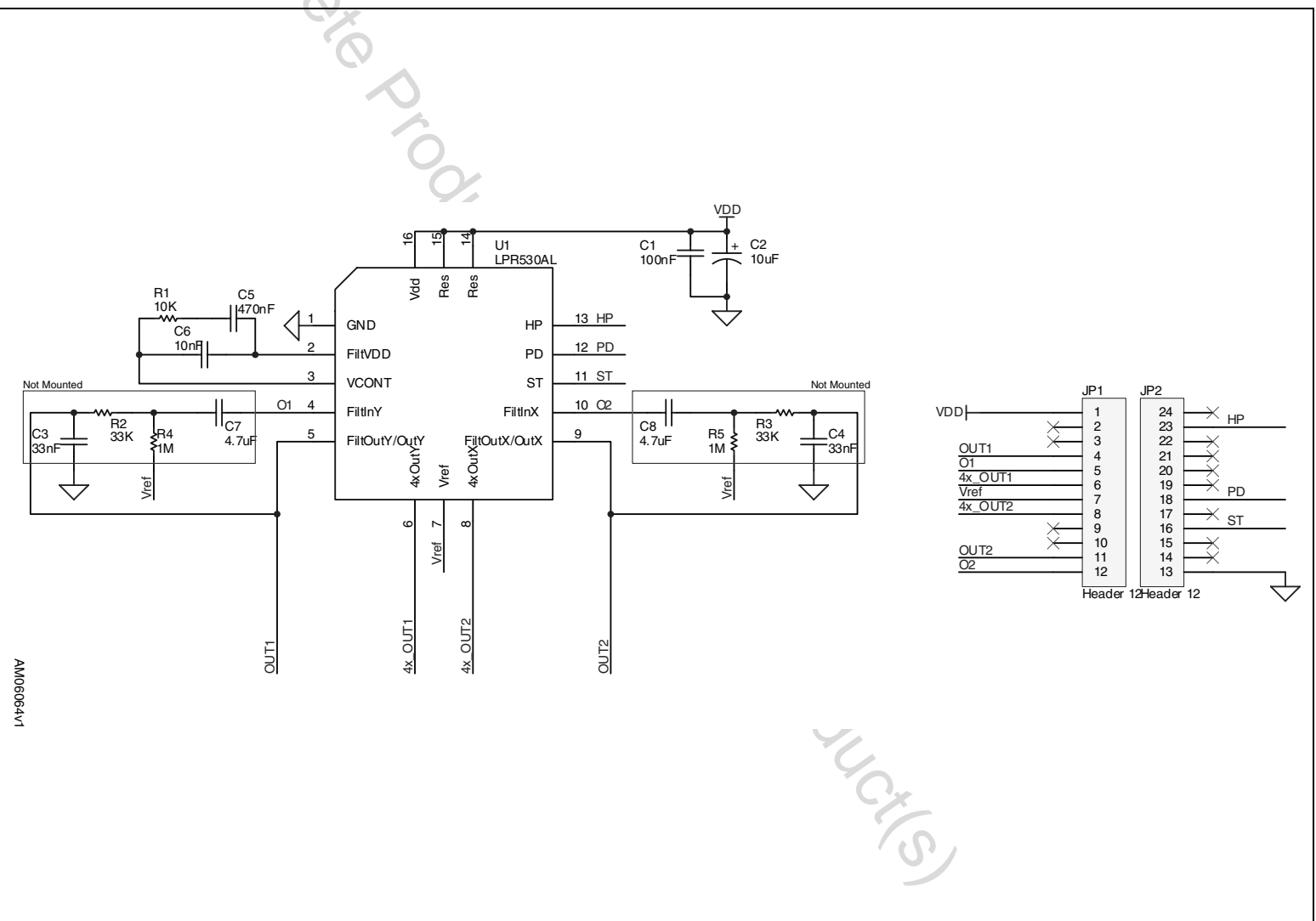
Figure 1. STEVAL-MK1044V1 adapter board schematic
