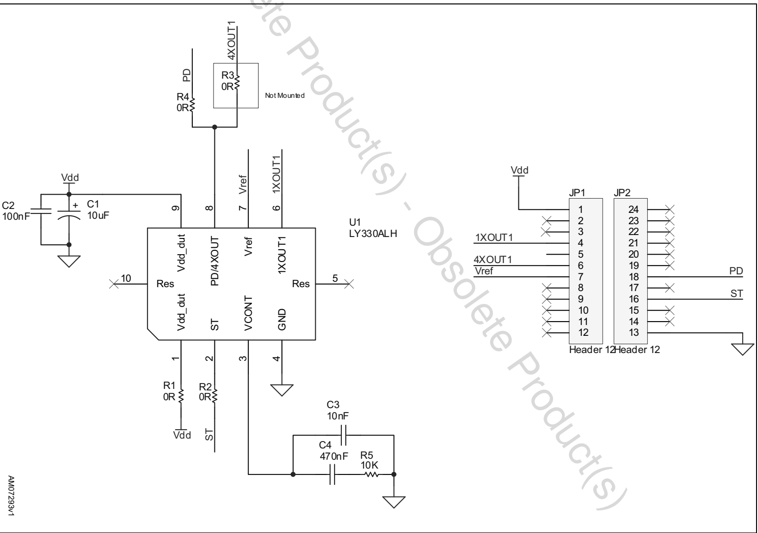
Figure 1. STEVAL-MK1074V1 circuit schematic
