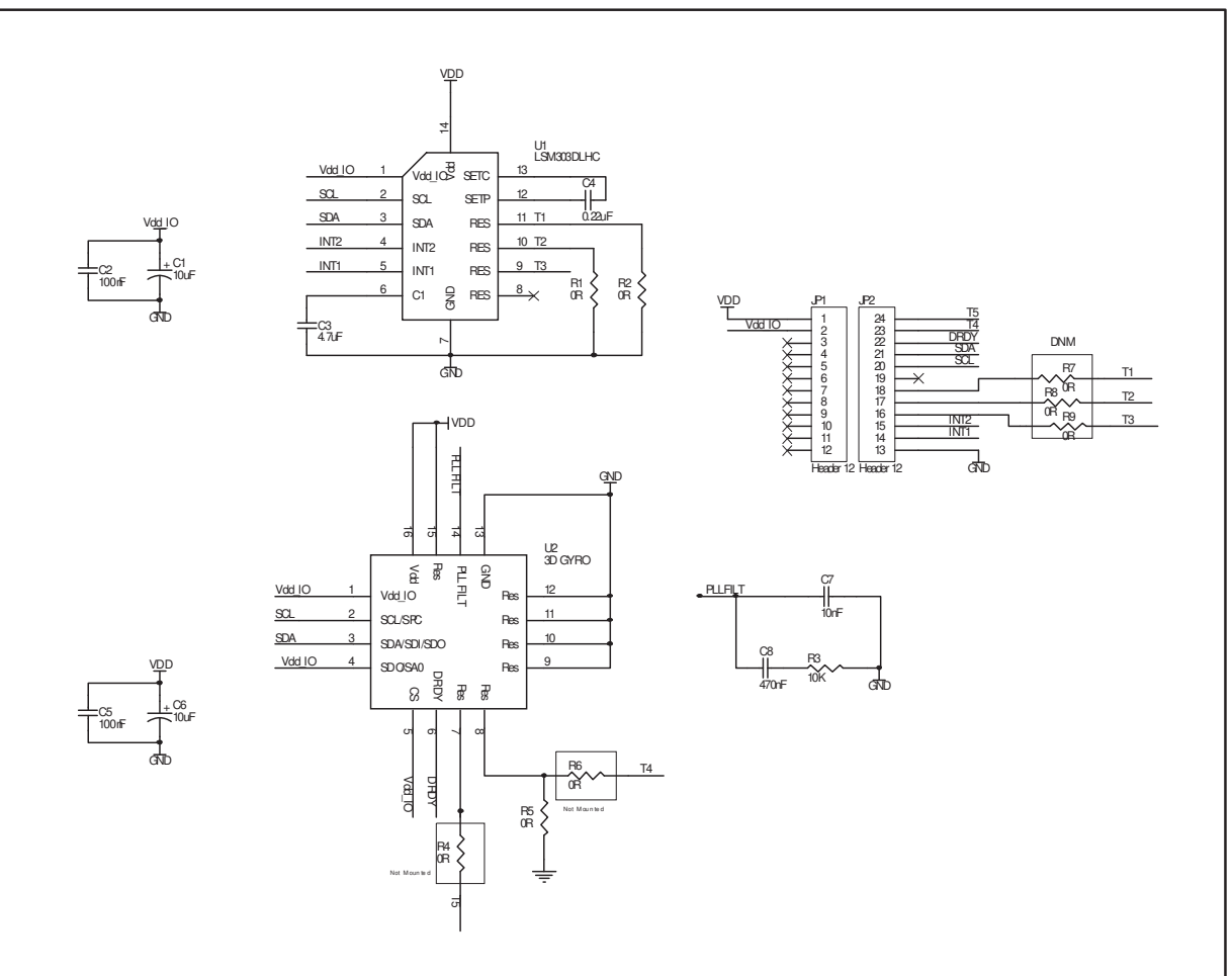
Figure 1 : STEVAL-MK1108V2 circuit schematic
