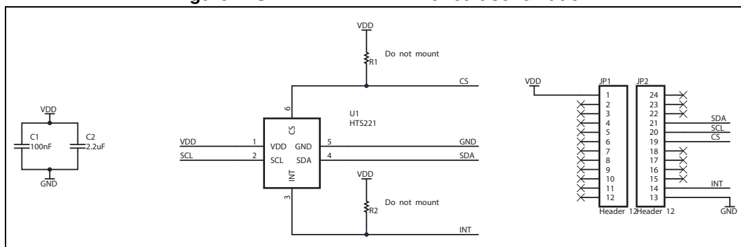
Figure 1. STEVAL- MKI141V2 circuit schematic
