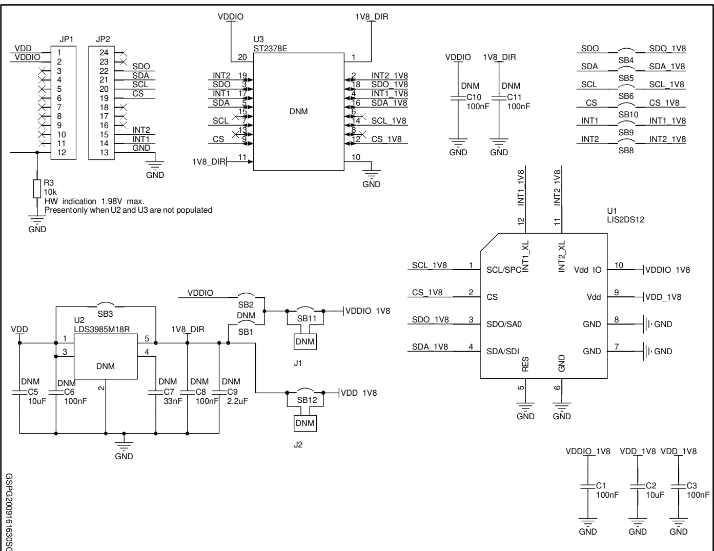
Figure 1: STEVAL-MK1174V1 circuit schematic
