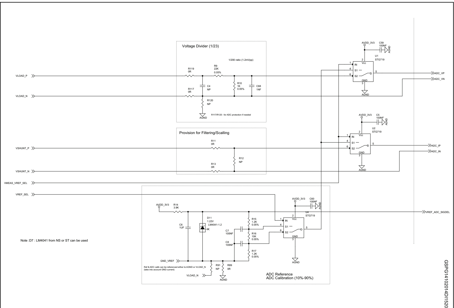
Figure 7. STEVAL-PCC019V1 circuit schematic (5 of 6)
