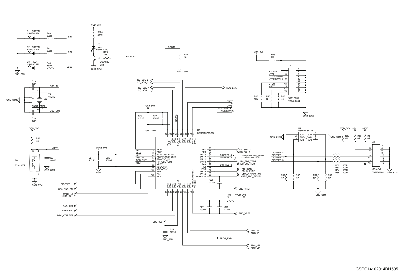
Figure 4. STEVAL-PCC019V1 circuit schematic (2 of 6)
