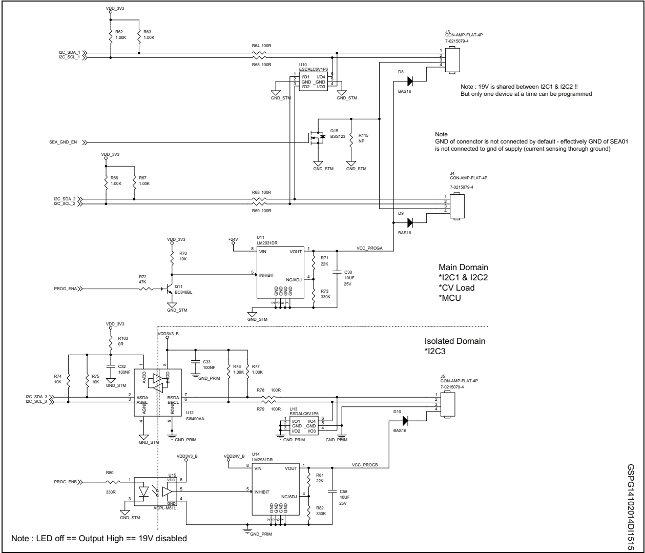
Figure 6. STEVAL-PCC019V1 circuit schematic (4 of 6)
