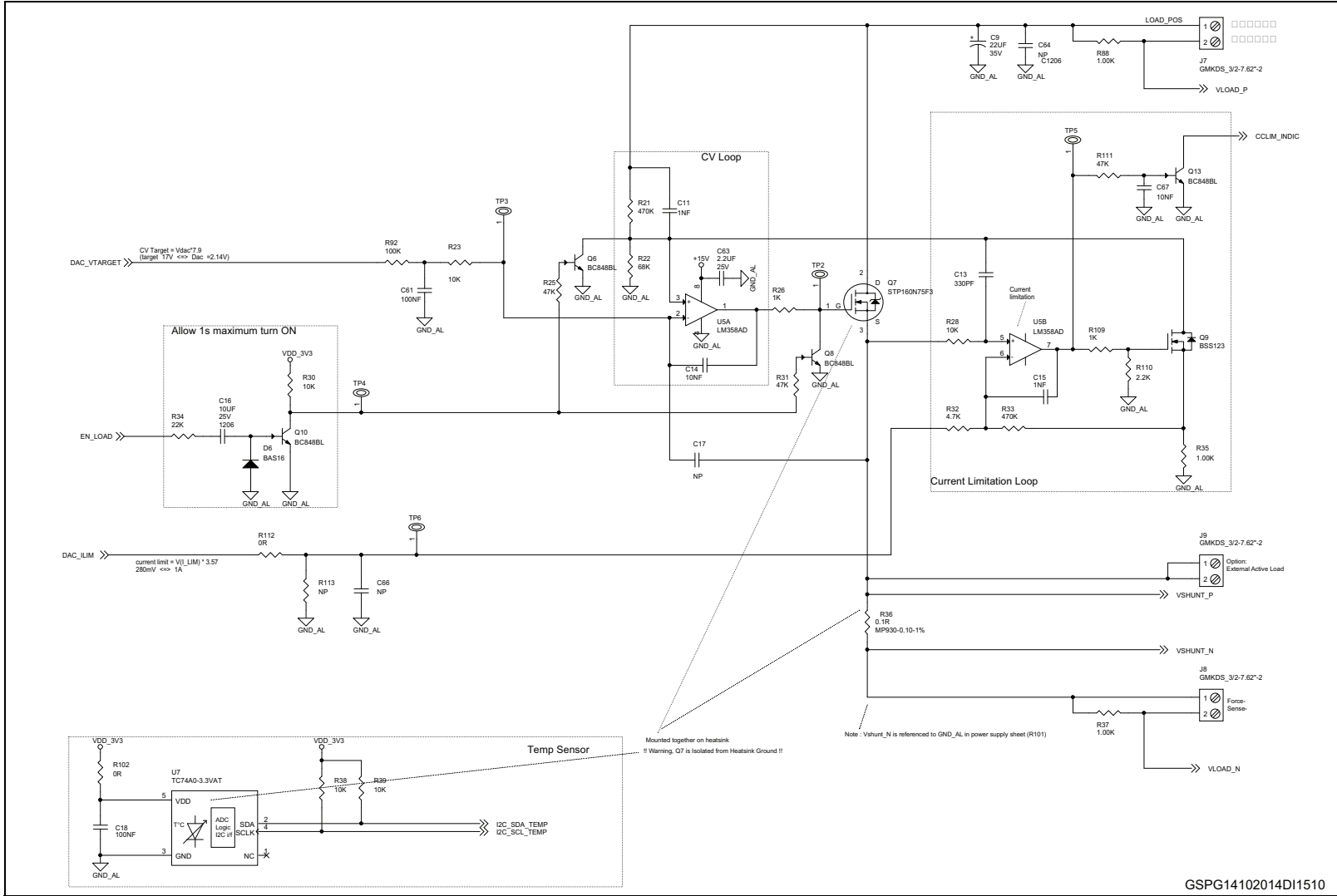
Figure 5. STEVAL-PCC019V1 circuit schematic (3 of 6)
