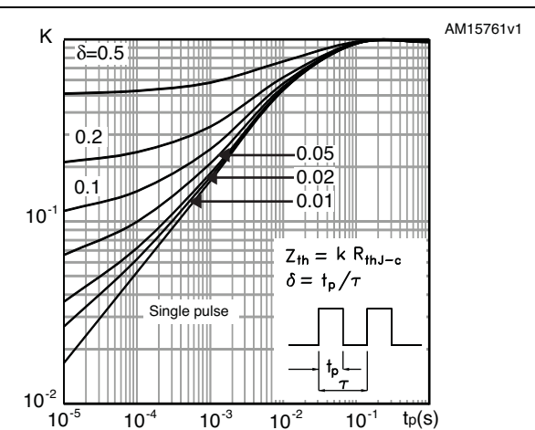
Figure 7. Thermal impedance for D 2 PAK and TO-220
