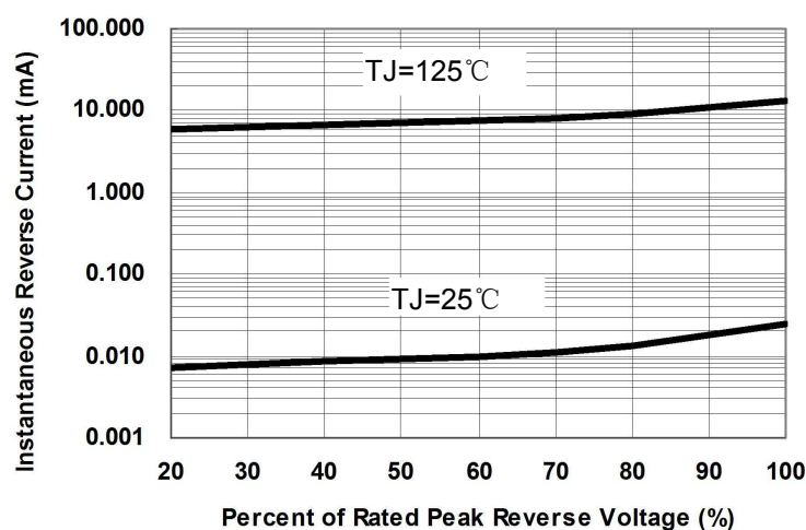
Fig.2-Typical Reverse Characteristics
