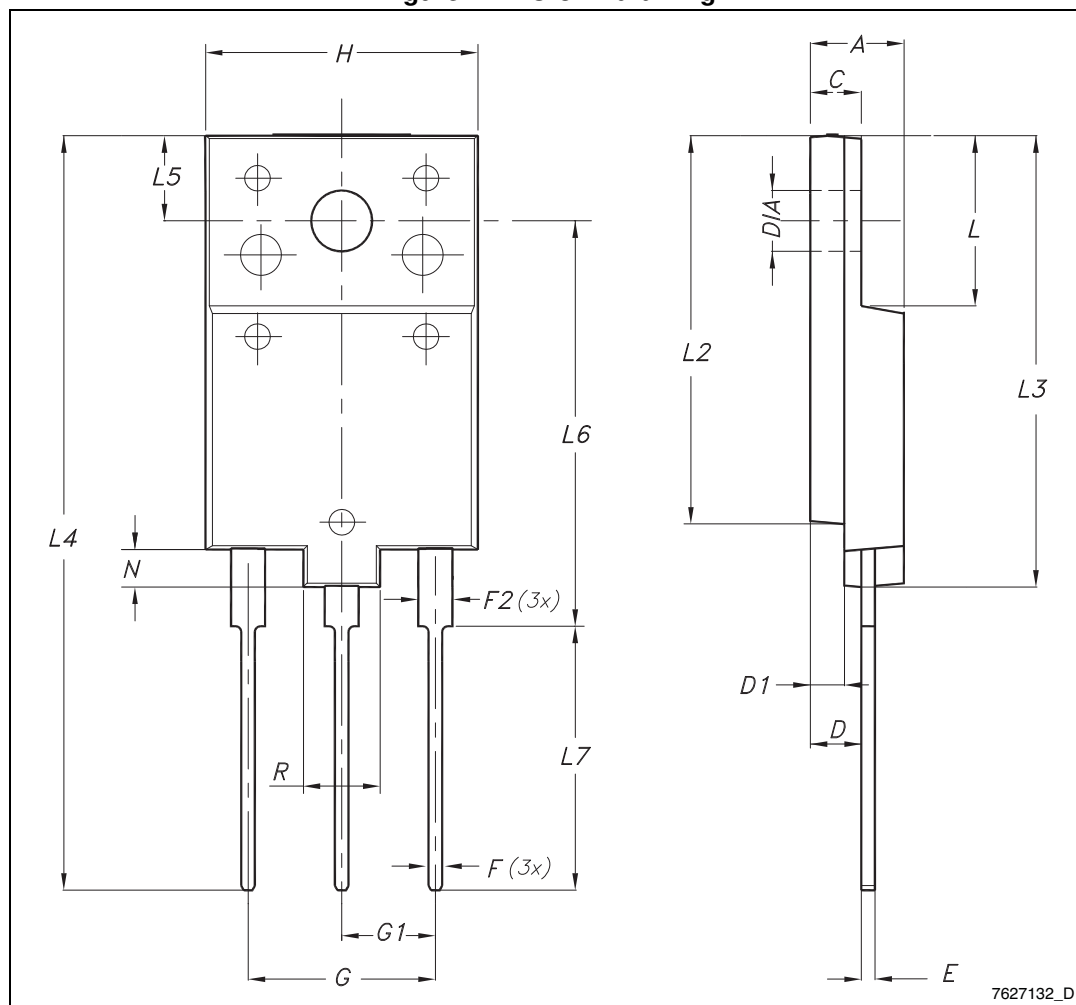
Figure 24. TO-3PF drawing
