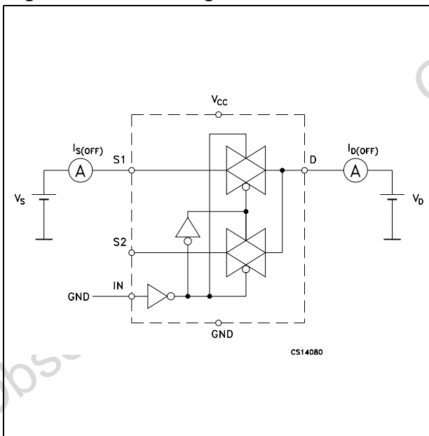
Figure 5. OFF Leakage
