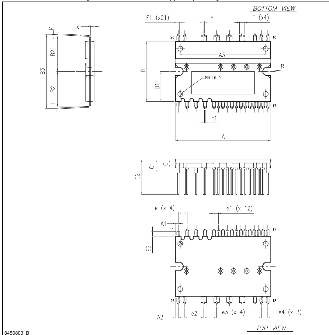
Figure 17. SDIP2F-26L type L package outline
