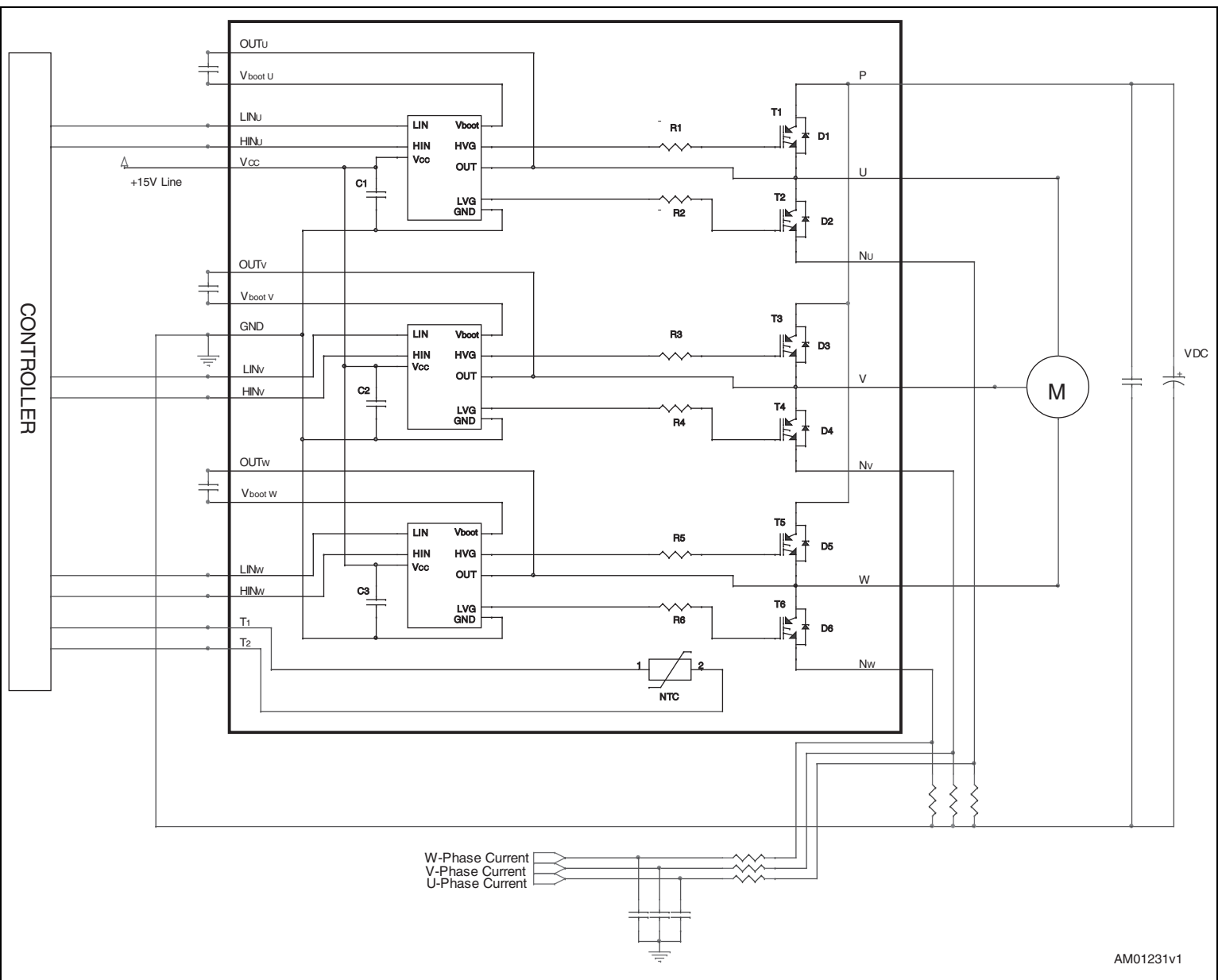
Figure 10. Typical application circuit
