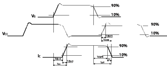
Figure 30: Switching waveform
