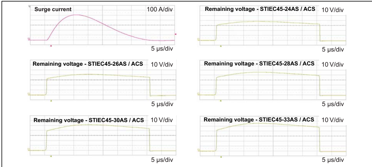
Figure 4. Clamping voltage at 500 A (1.2/50 \mu s - 8/20 \mu s)
