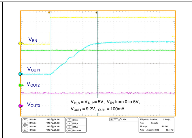
Figure 31. Enable transient
