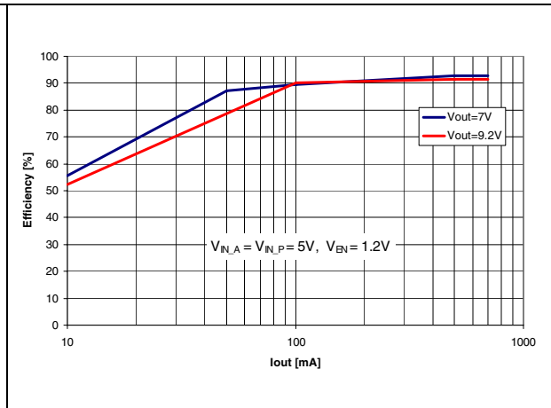
Figure 27. Efficiency step-up vs. output current
