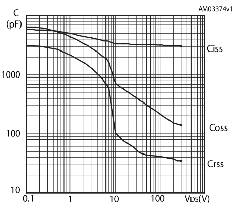
Figure 10: Capacitance variations
