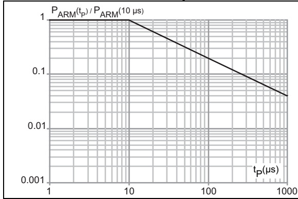
Figure 3. Normalized avalanche power derating versus pulse duration (pulse > 10 \mu s, T_j < 150 °C)
