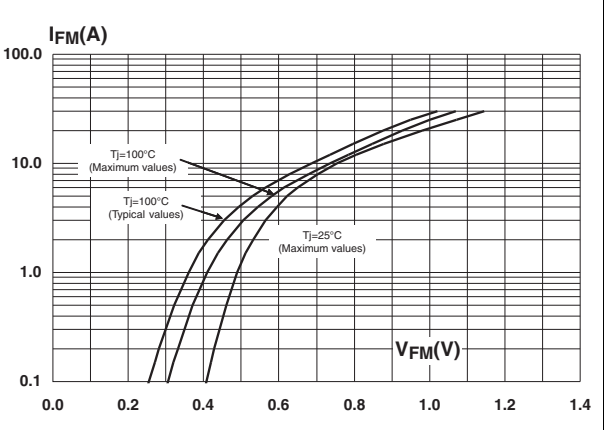
Figure 8. Forward voltage drop versus forward current (high level)
