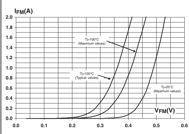
Figure 7. Forward voltage drop versus forward current (low level)
