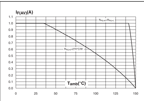
Figure 2. Average forward current IF(AV)(A) versus ambient temperature (delta = 0.5)
