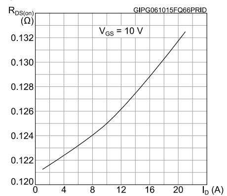
Figure 11: Static drain-source on-resistance
