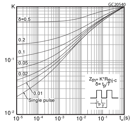
Figure 3: Thermal impedance for D 2 PAK
