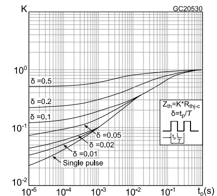
Figure 7: Thermal impedance for TO-247
