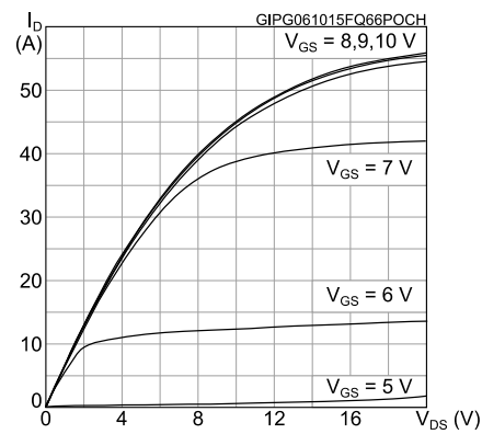
Figure 8: Output characteristics
