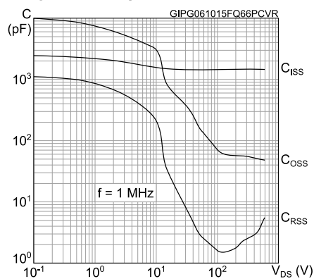
Figure 12: Capacitance variations
