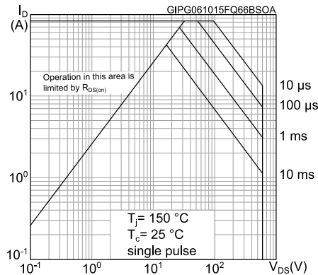
Figure 2: Safe operating area for D 2 PAK
