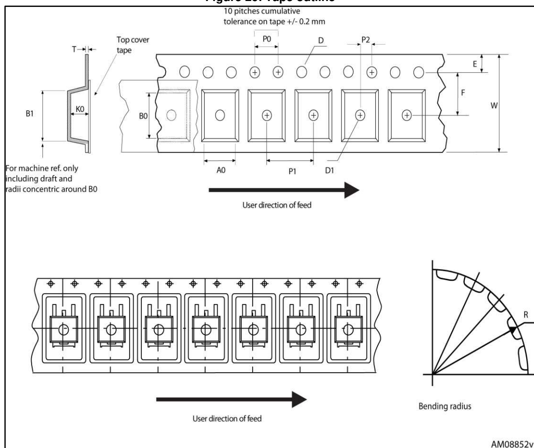
Figure 26: Tape outline
