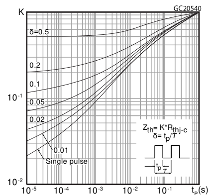
Figure 5: Thermal impedance for TO-220
