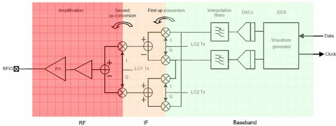
Figure 17. SX1211 Simplified Transmitter Block Schematic Diagram
