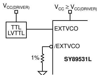
Figure 5a. 3.3V "TTL"
