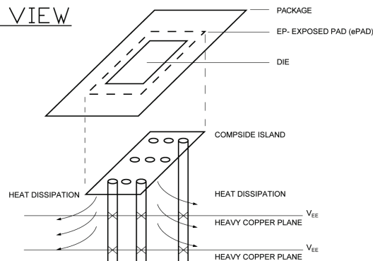
PCB Thermal Consideration for 16-Pin QFN Package (Always solder, or equivalent, the exposed pad to the PCB)
