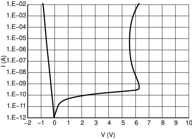
Figure 1. IV Characteristics
