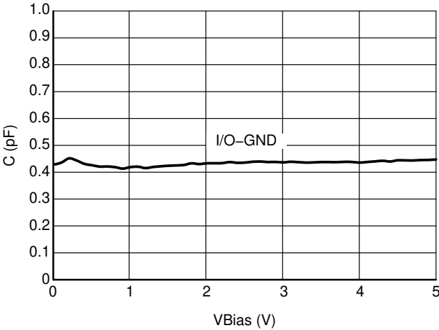
Figure 2. CV Characteristics
