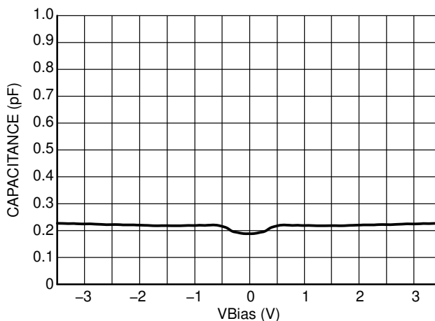
Figure 11. CV Characteristics
