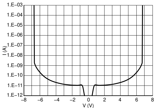
Figure 10. IV Characteristics
