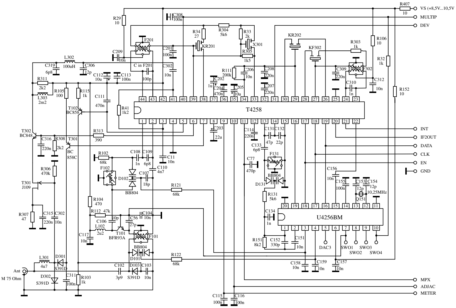
Figure 6. Application board schematic
