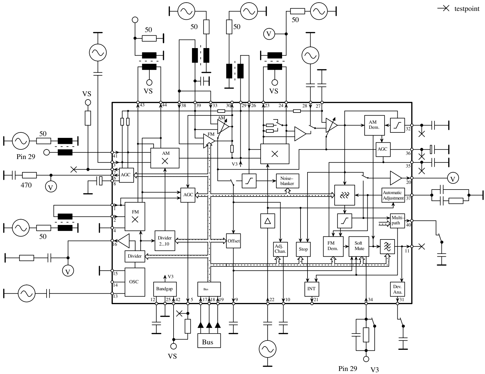
Figure 5. Test circuit
