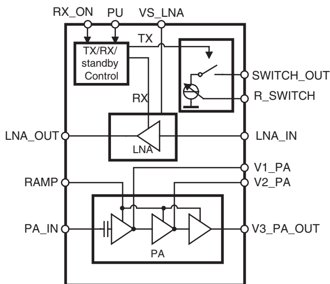
Figure 1-1. Block Diagram
