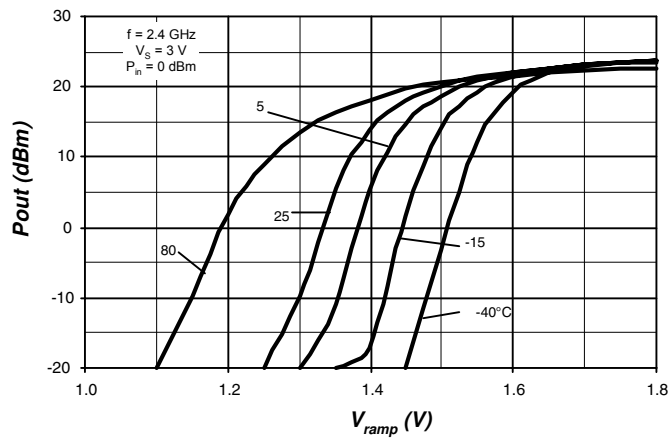
Figure 9-15. PA (PSSO20, QFN20): P_{out} versus V_{RAMP} and Temperature
