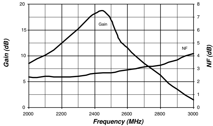
Figure 9-2. LNA (N20): Gain and Noise Figure versus Frequency
