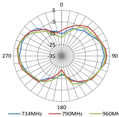
E Plane - 734 - 960MHz
