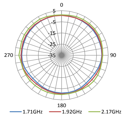
H Plane - 1710 - 2170MHz
