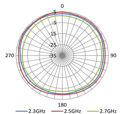
H Plane - 2300 - 2700MHz
