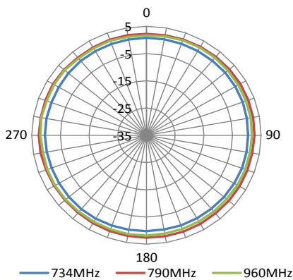
H Plane - 734 - 960MHz
