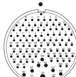
48-5 90 #16(A-BL,BN-BT,BW,BX) 1 #8(CD) 9 #12(BM,BU,BV,BY-CC,CE) A
