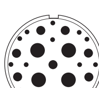
40-10 16 #16(A,B,E-H,M,N,P Q,V-Y,b,c) 9 #8(C,D,I,L,O,R,U,Z,a) 4 #4(K,J,S,T) A
