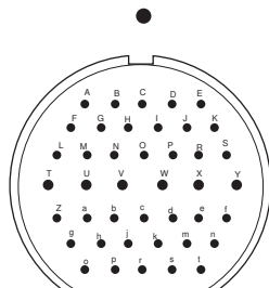
44-1 36 #16(A-S,Z-t) 6 #12(T-Y) D
