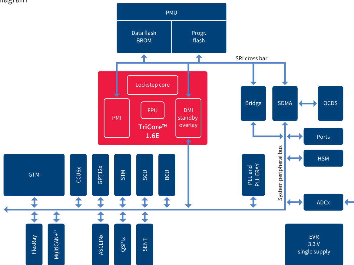
Block diagram
