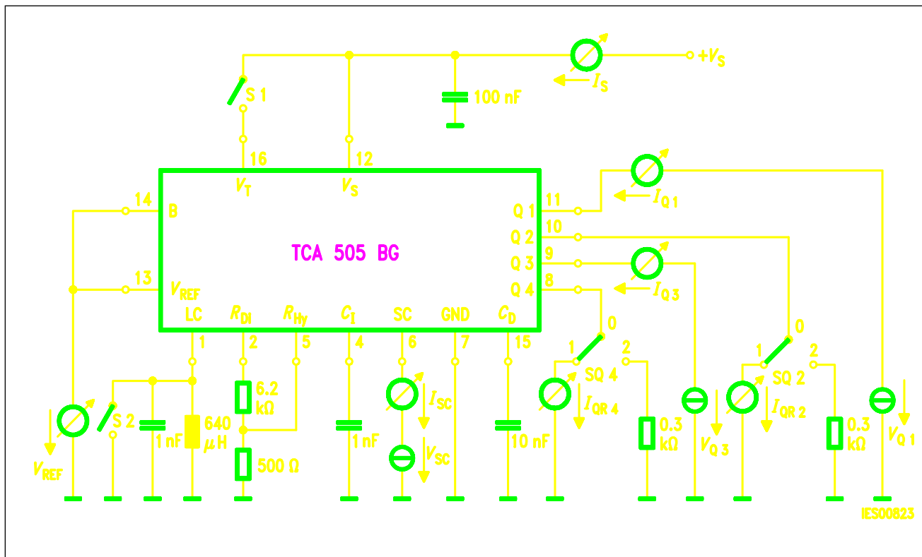
Test Circuit 1
