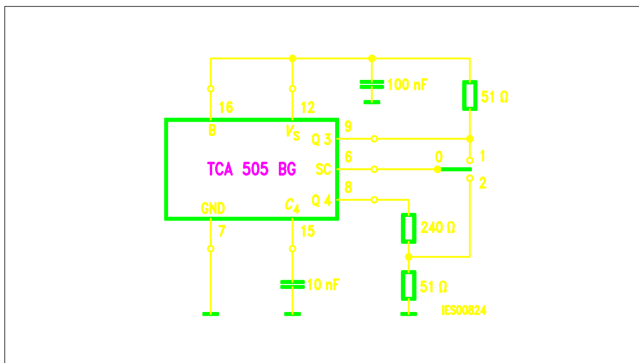
Test Circuit 2
