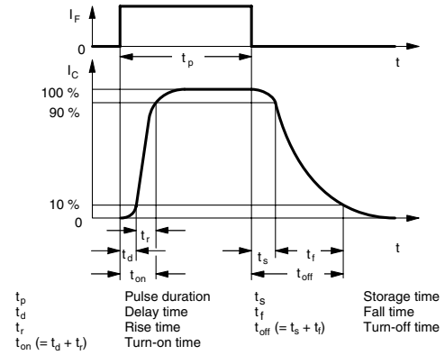
Fig. 4 - Switching Times
