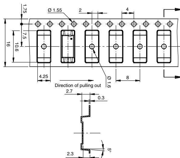
Fig. 7 - Tape Packing
