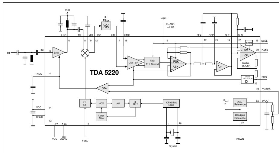
Figure 2 Block Diagram
