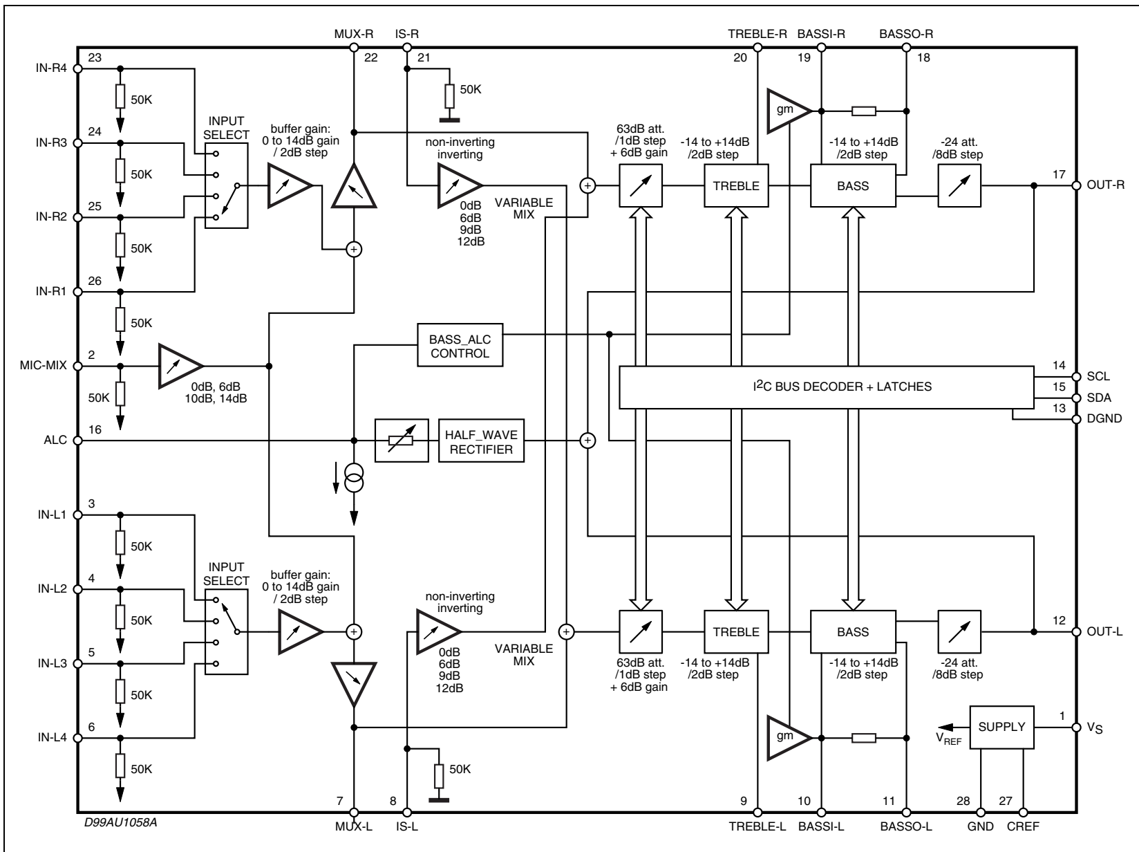
Figure 3. BLOCK DIAGRAM
