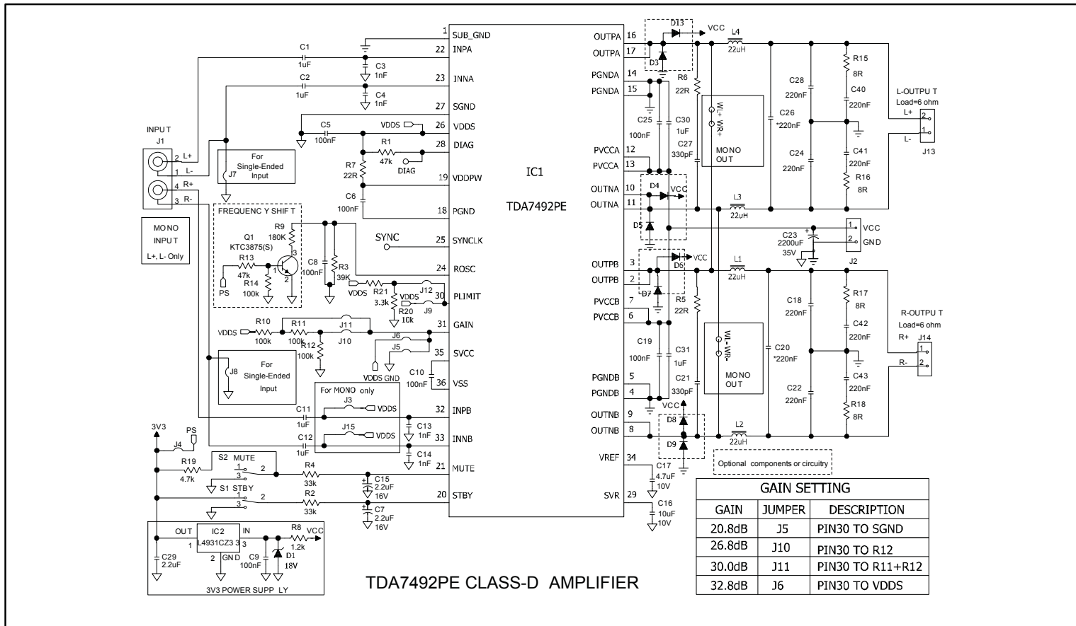
Figure 7: Application circuit
