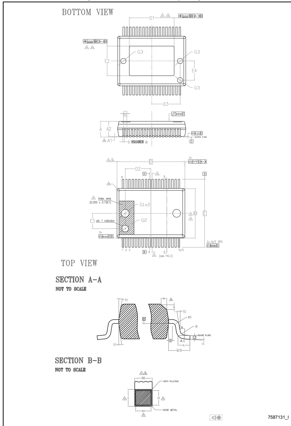
Figure 17: PowerSSO-36 EPD package outline
